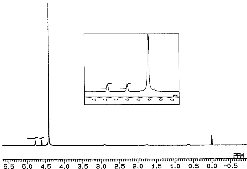
FIG. 2—Variable temperature ^1\text{H} NMR spectrum of liquid sample taken at 60^\circ\text{C} .
